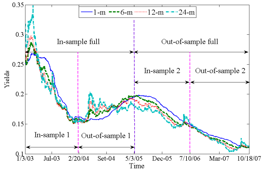
Figure 3: Time series of some yields.
