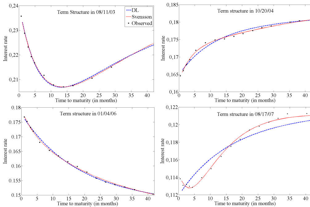
Figure 4: Pictures of term structure cross-sections.
