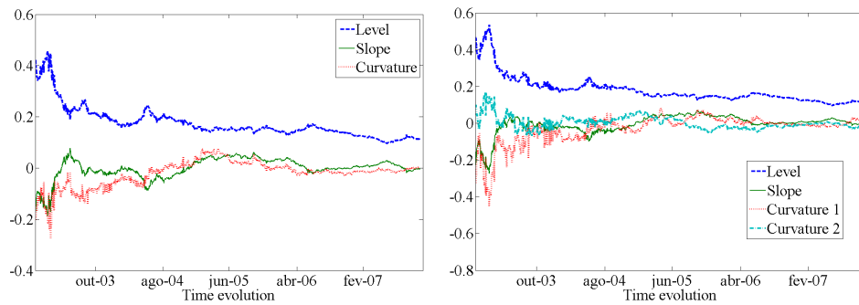
Figure 6: Term structure movements
