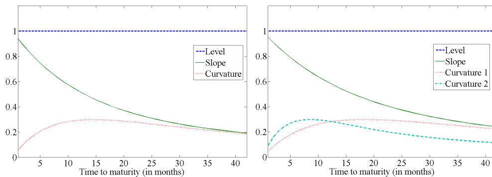
Figure 1: Loadings of the DL and Svensson models.
