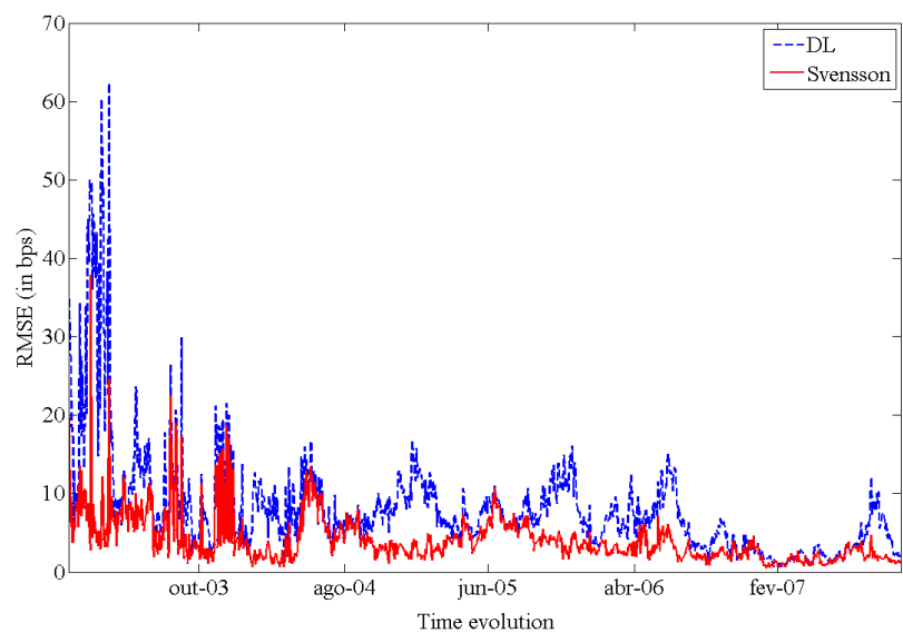
Figure 5: RMSE for in-sample fit
